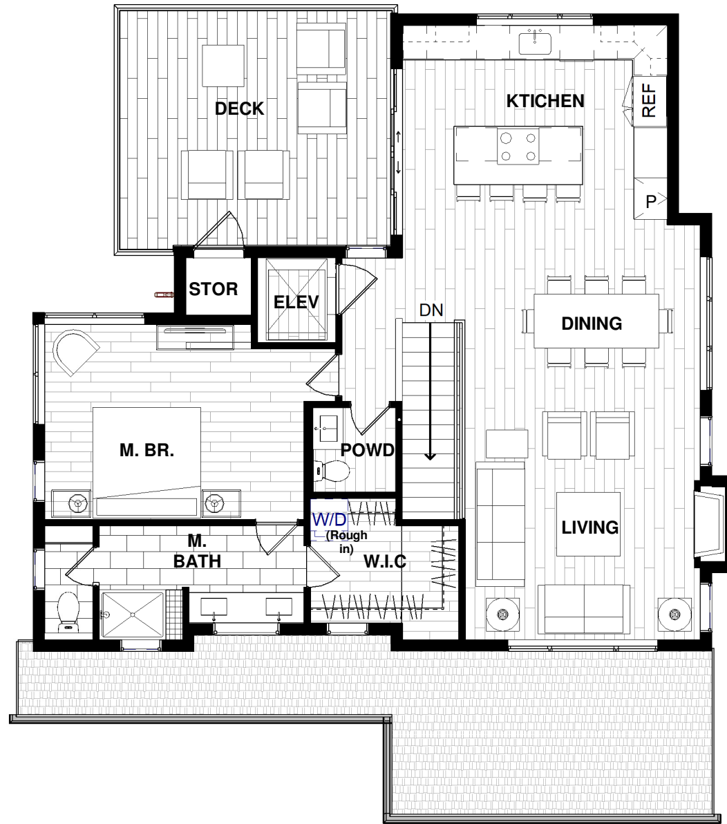
2ND LEVEL 1/8" = 1'-0"
