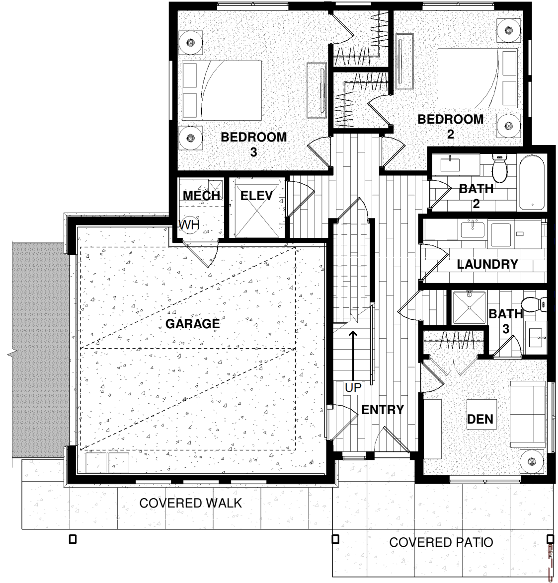
1ST LEVEL 1/8" = 1'-0"
